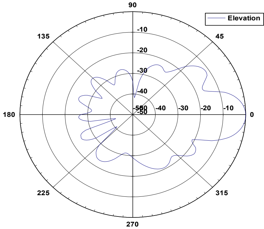
19 3030 Elevation Pattern
