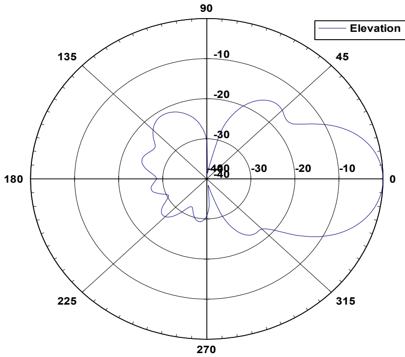
19 4040H Elevation Pattern
