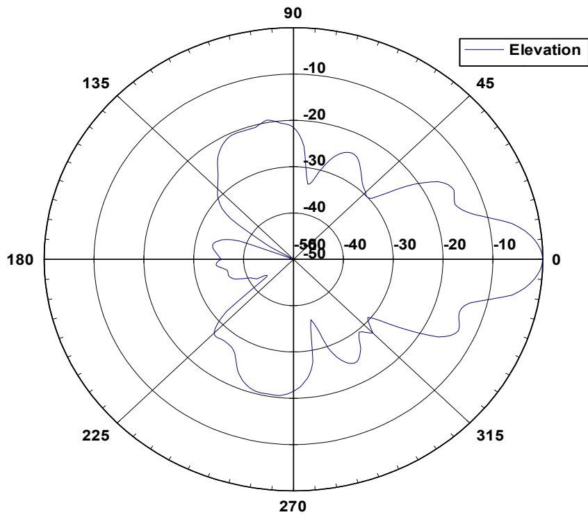
19 SD15 Elevation Pattern
