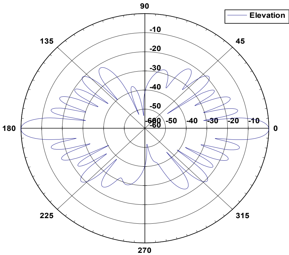
19 2360 Elevation Pattern
