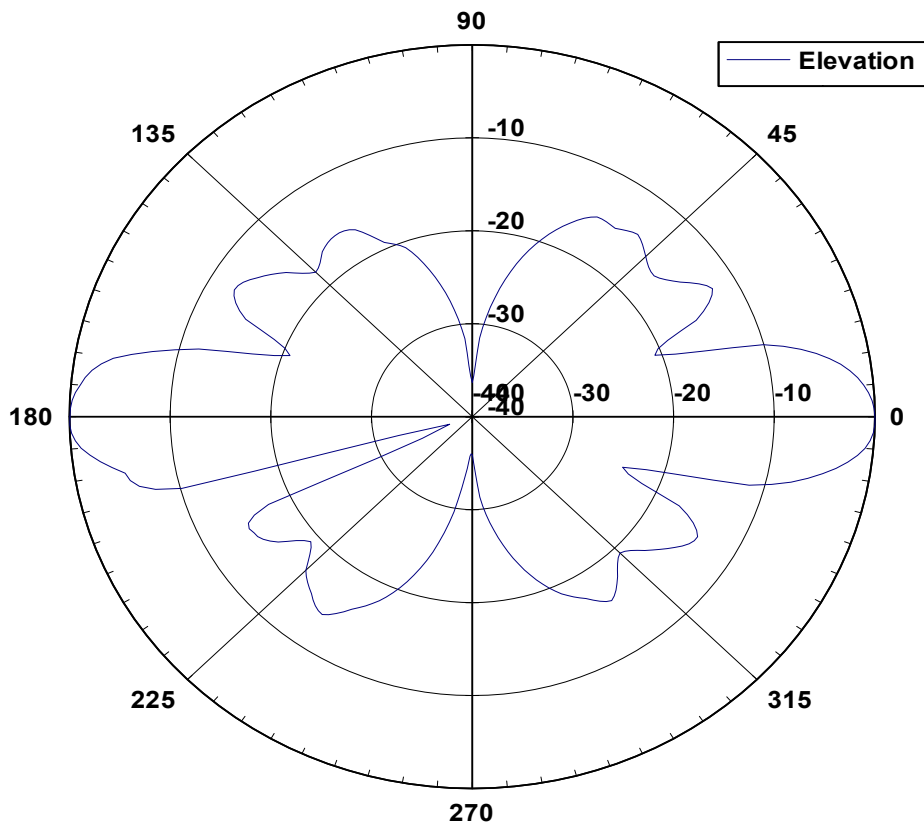
19 1360 Elevation Pattern
