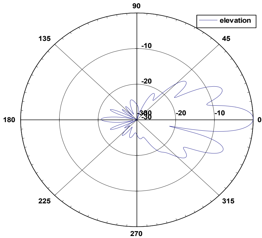
1.7GHz 9015 Elevation Pattern
