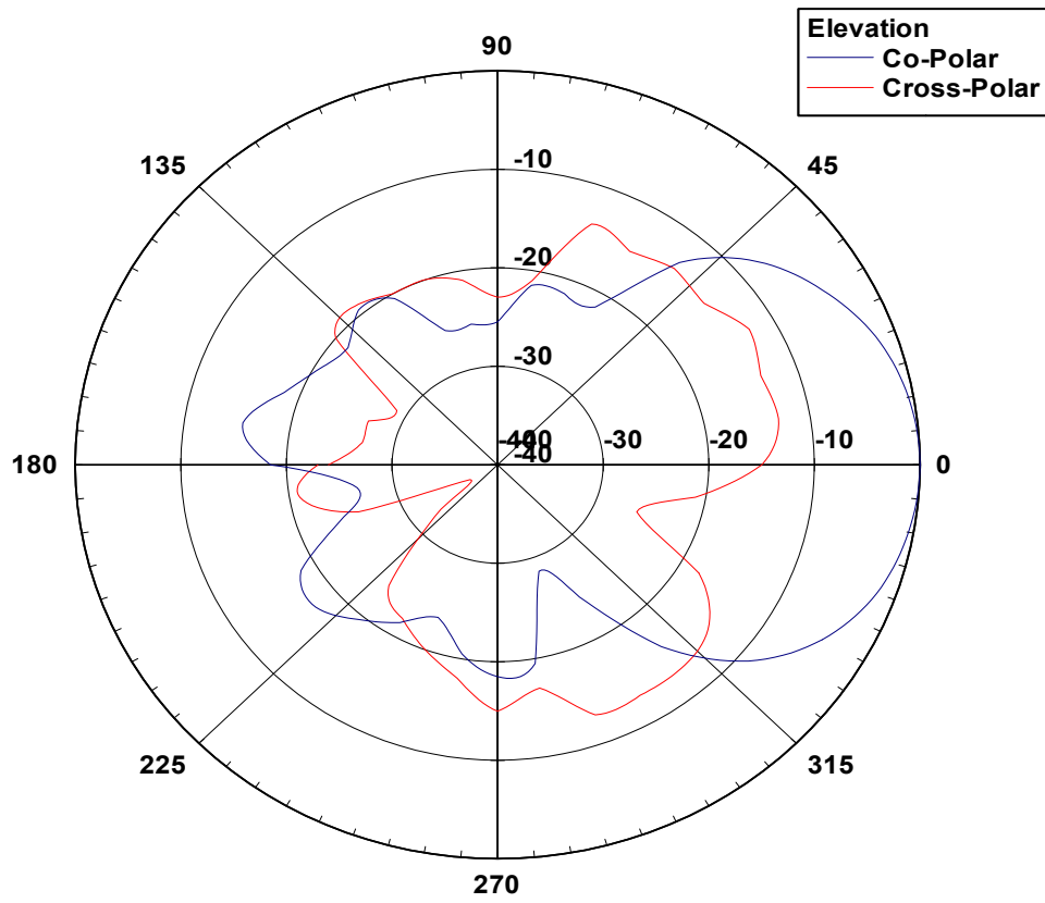
14 8080H Elevation Pattern
