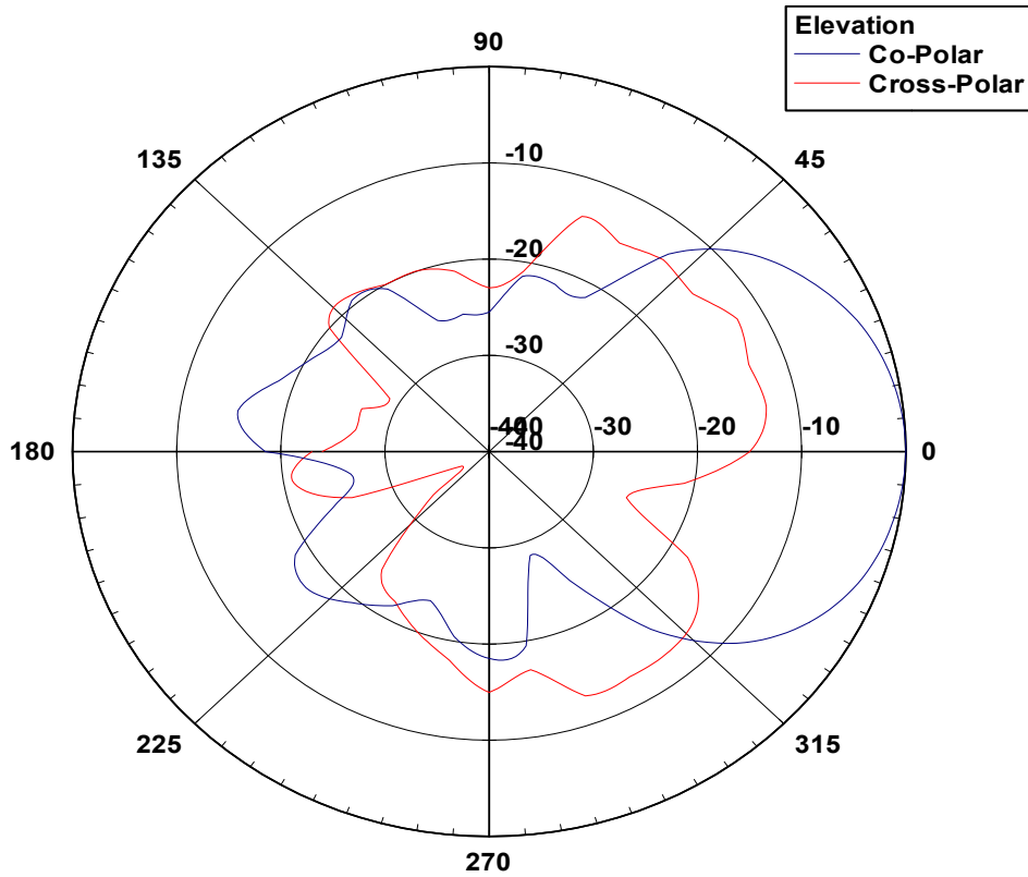
14 8080 Elevation Pattern
