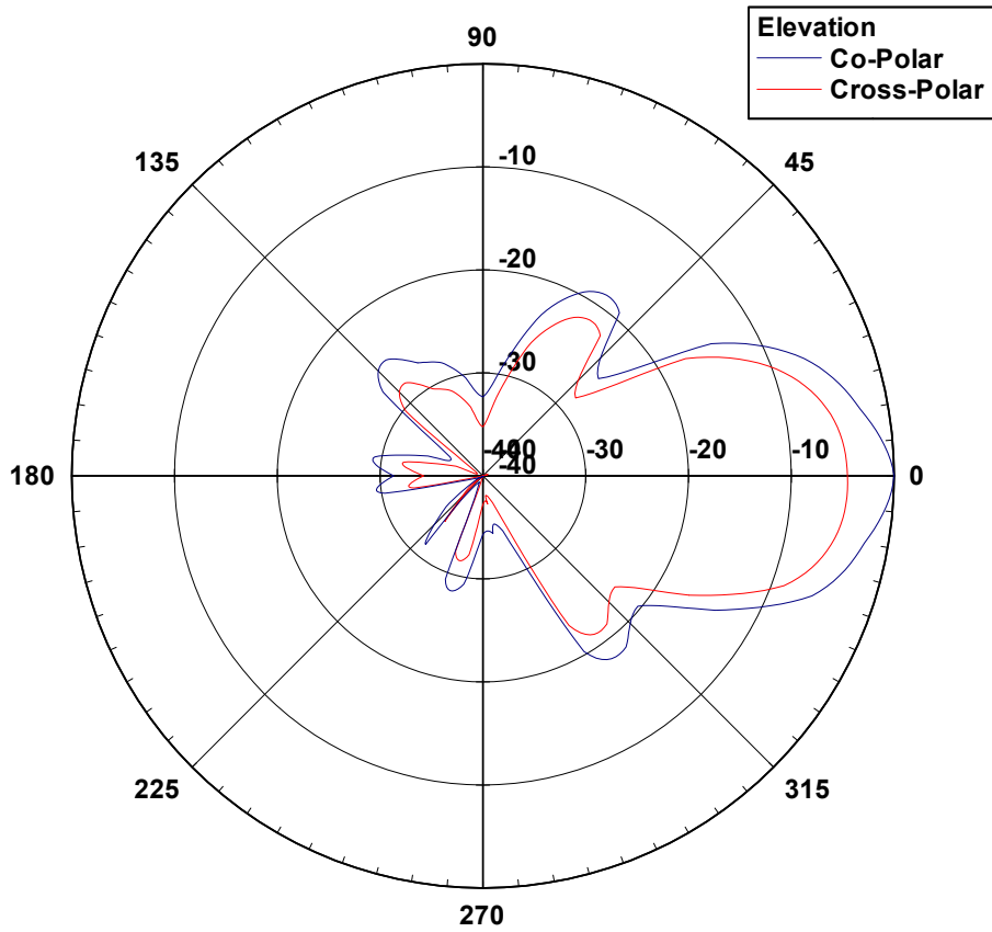
14 4040 Elevation Pattern
