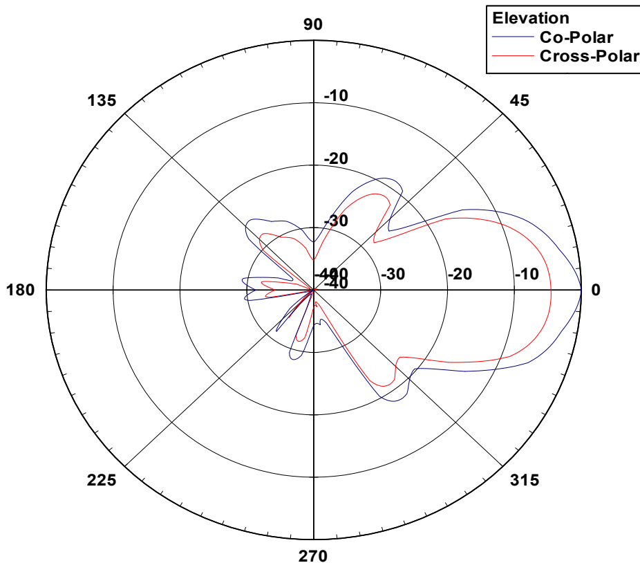
12 4040H Elevation Pattern
