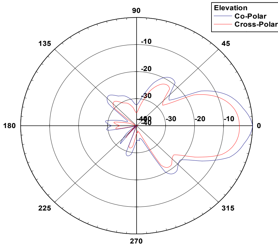
12 4040 Elevation Pattern
